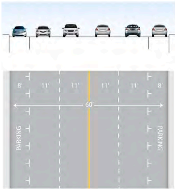
Existing 60'-wide avenue or boulevard
