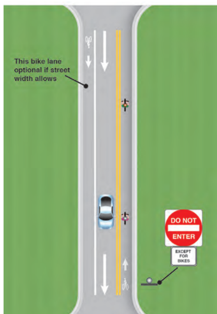
Contra-flow bike lane design (Credit: Michele Weisbart)
