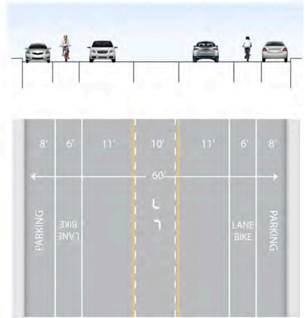
Option 1: Reduce travel lanes and add bike lanes
