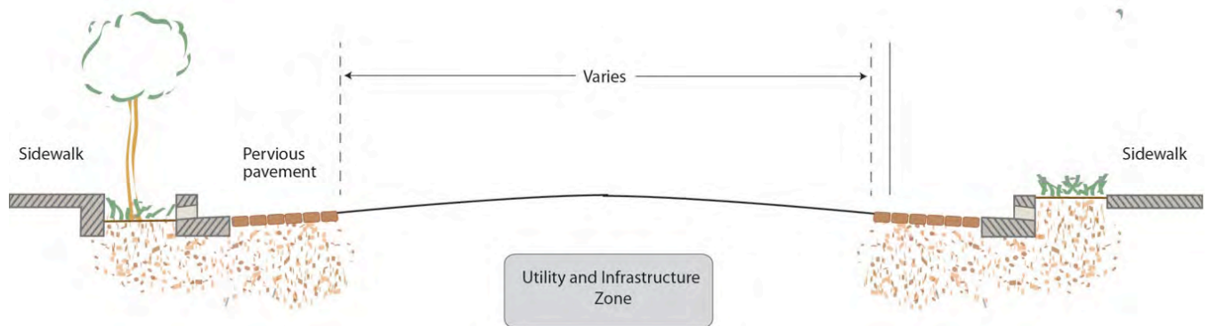
Street section elevation illustrating placement of permeable paving (Credit: Marty Bruinsma)
