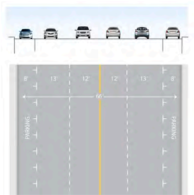
Existing 66'-wide boulevard
