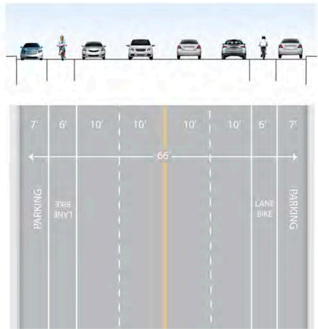
Narrow travel lanes to add bike lanes
