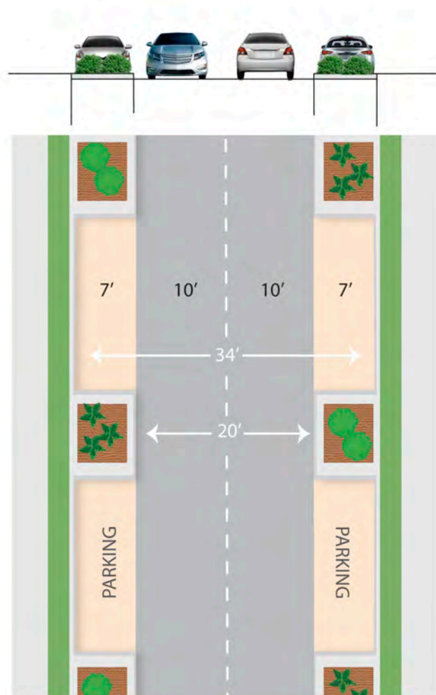
Residential street with inset parking
