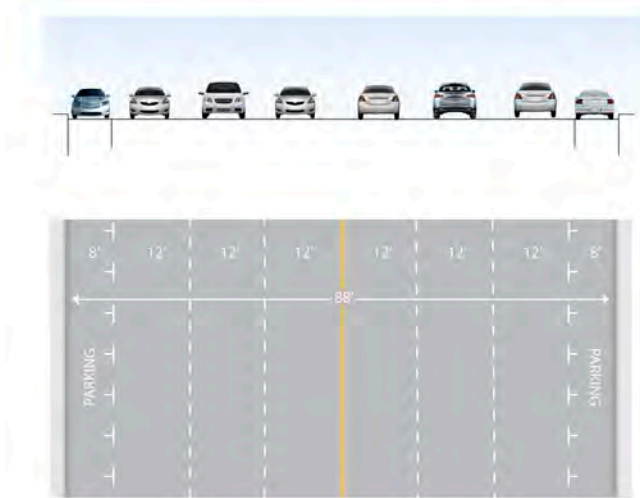
Existing 88'-wide boulevard
