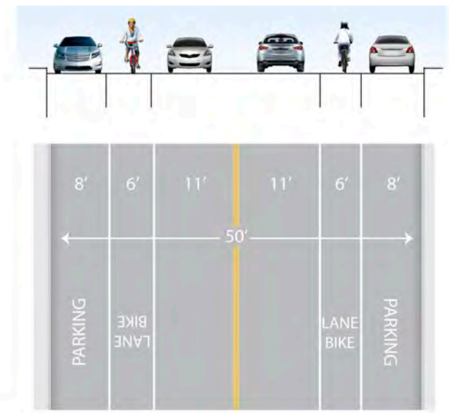
Option 1: Restripe to add bike lanes
