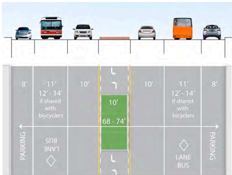
Boulevard with bus lanes
