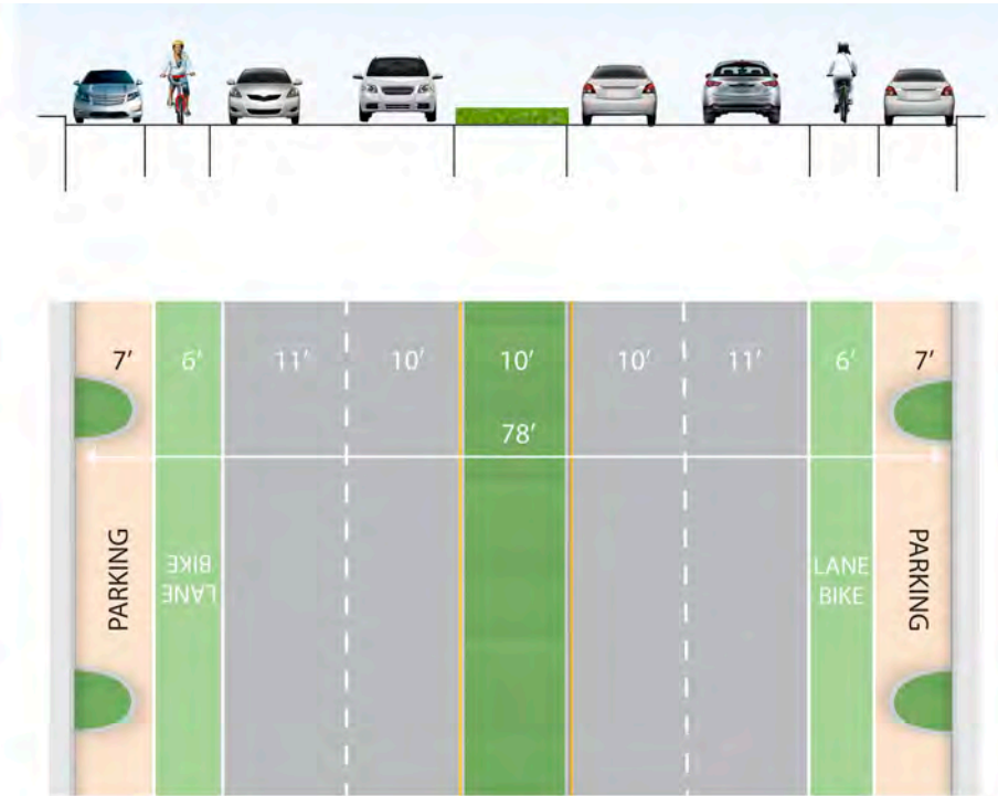
Boulevard with colored bike lanes and inset parking
