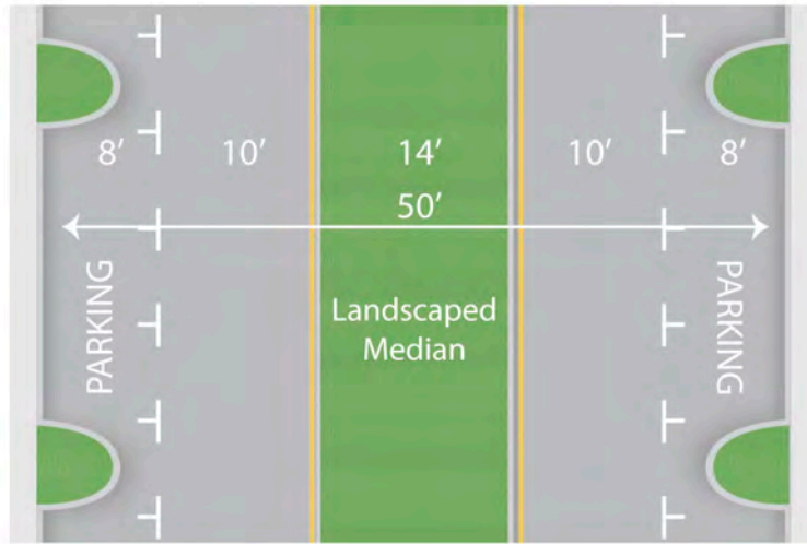
Option 2: Add median
