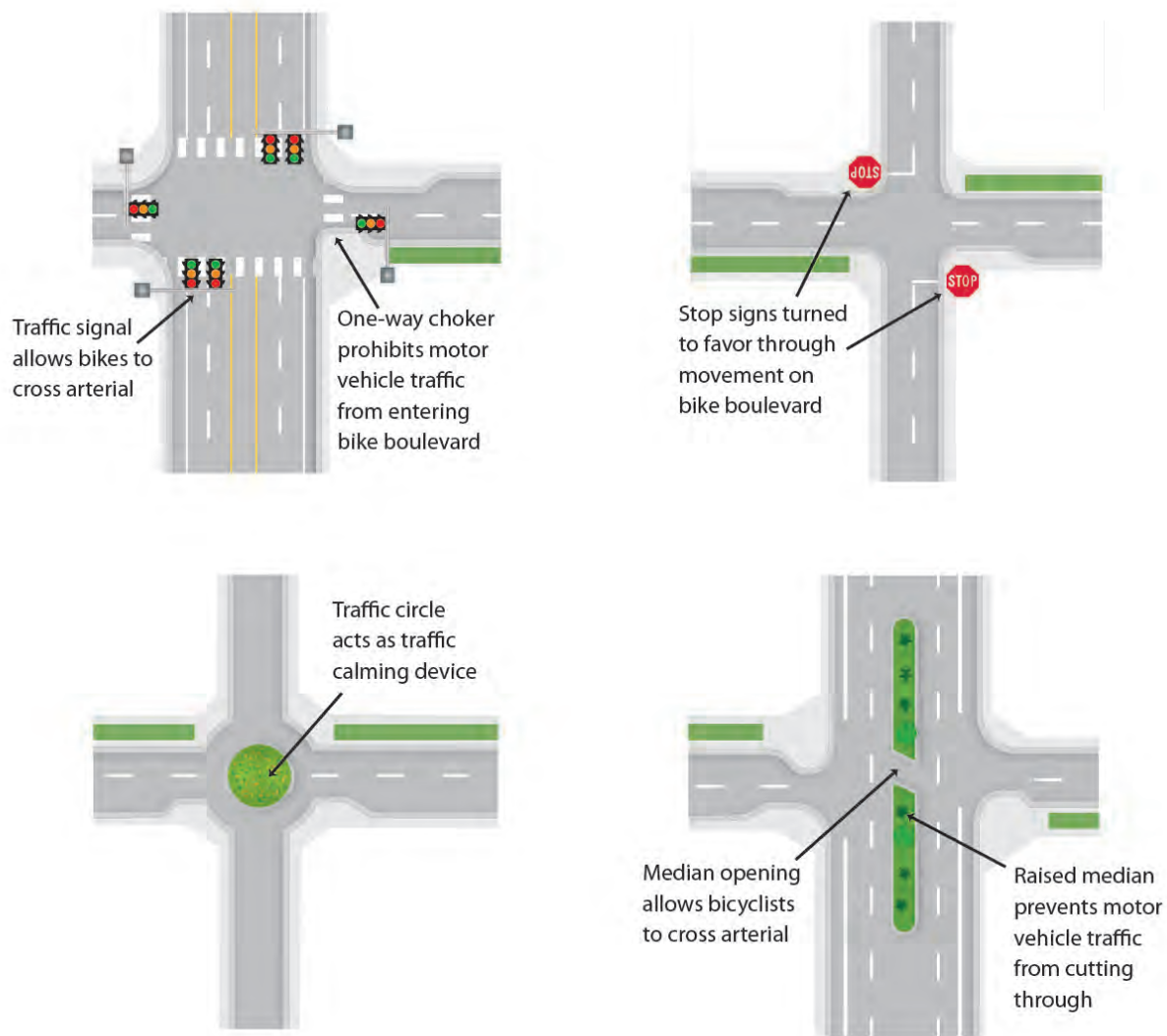
Components of bike boulevards (Credit: Michele Weisbart)
