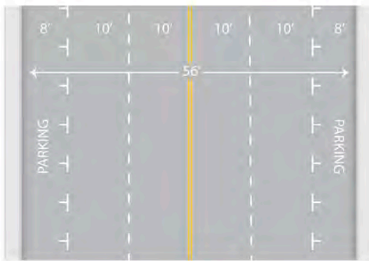
Existing 56'-wide main street
