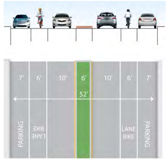
Avenue with median
