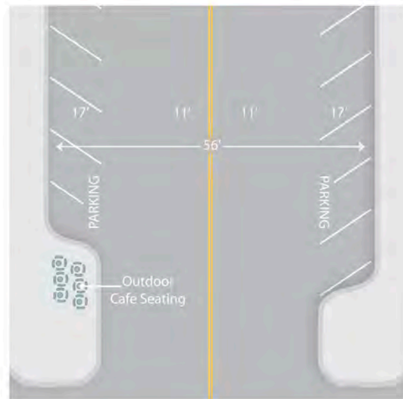
Reduce travel lanes and add reverse-in angled parking with curb extensions large enough for café seating
