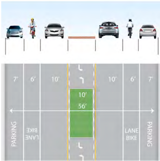
Avenue with medians interspersed with turn lanes
