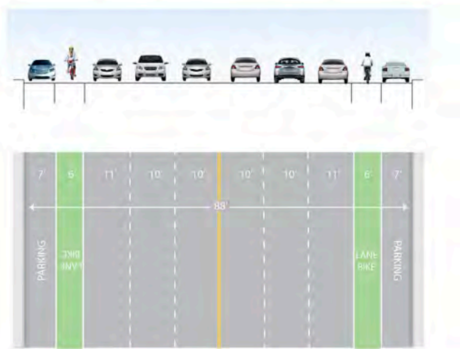
Narrow travel lanes to add colored bike lanes
