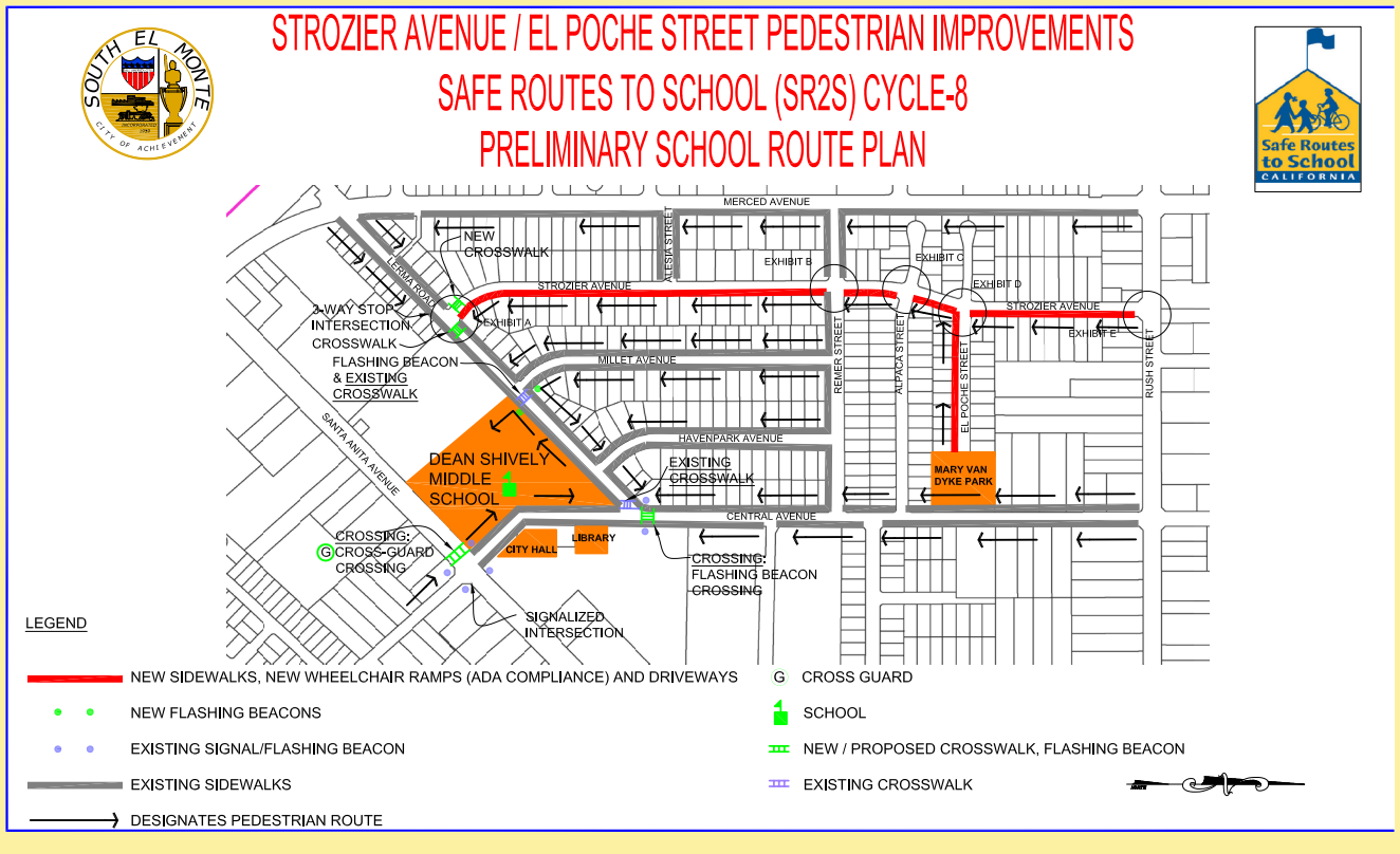
Figure 7-5 Shively Middle School Preliminary School Route Plan
