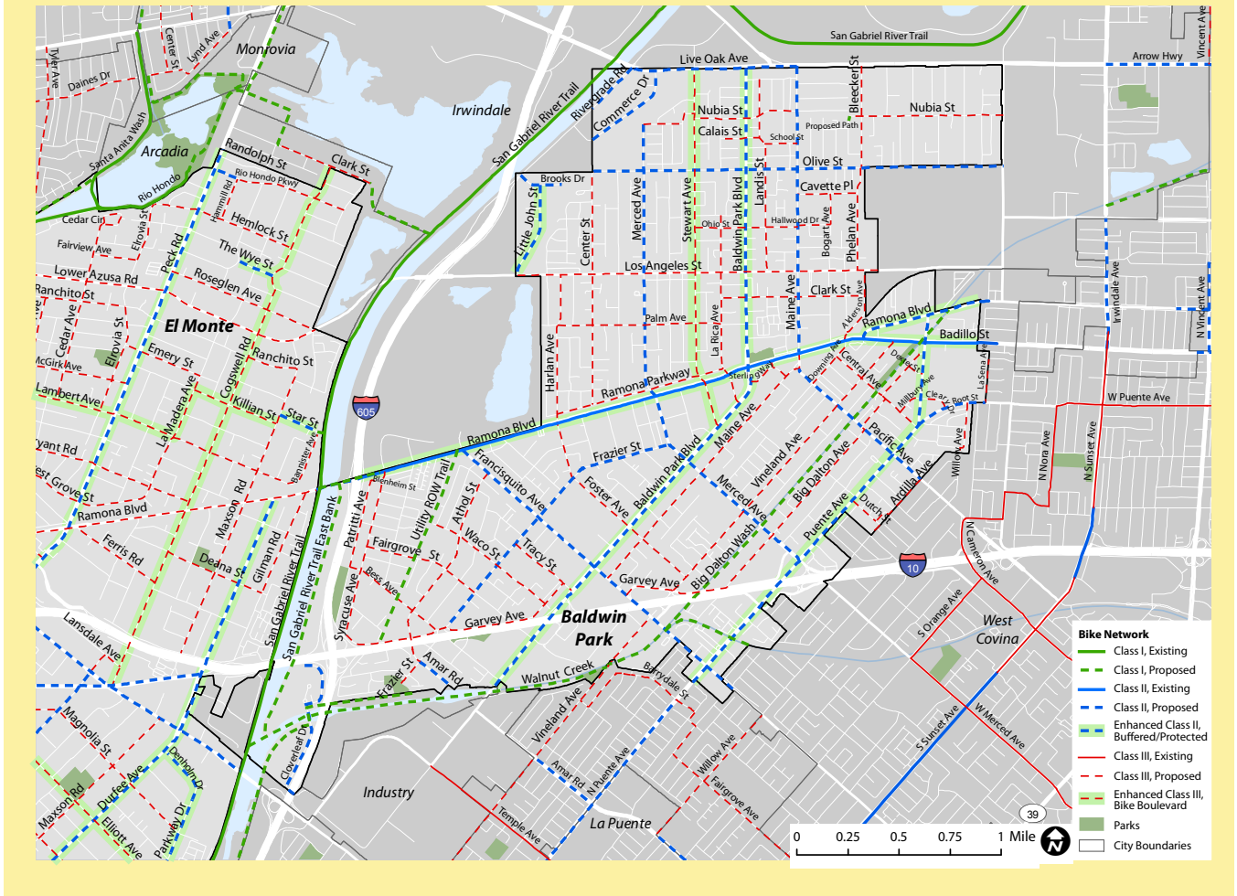
Figure 3-11 Baldwin Park Recommended Bikeway Network
