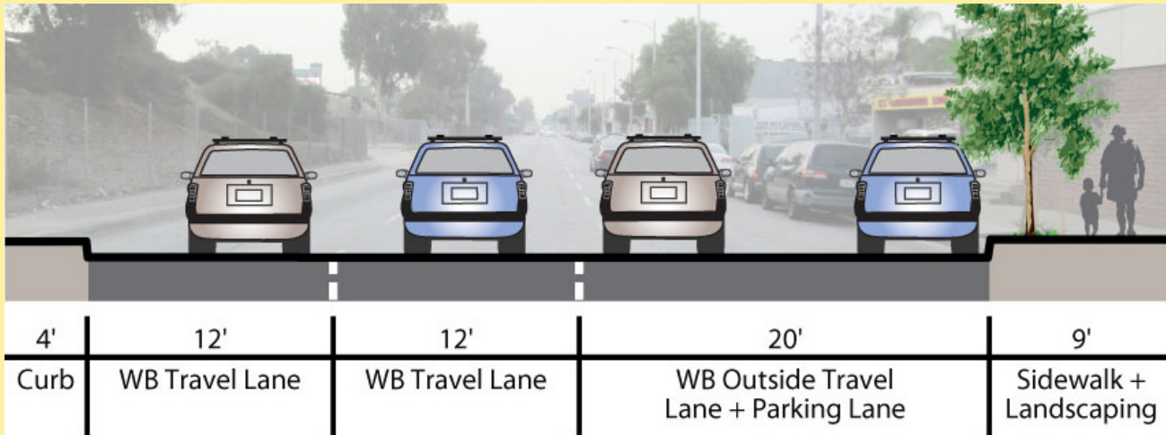
Existing Street Cross-Section
