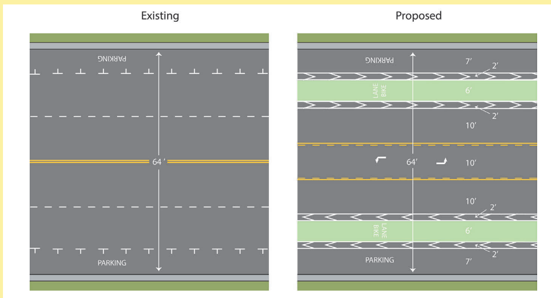
Figure 3-2 Proposed lane reconfiguration along Frazier Street
