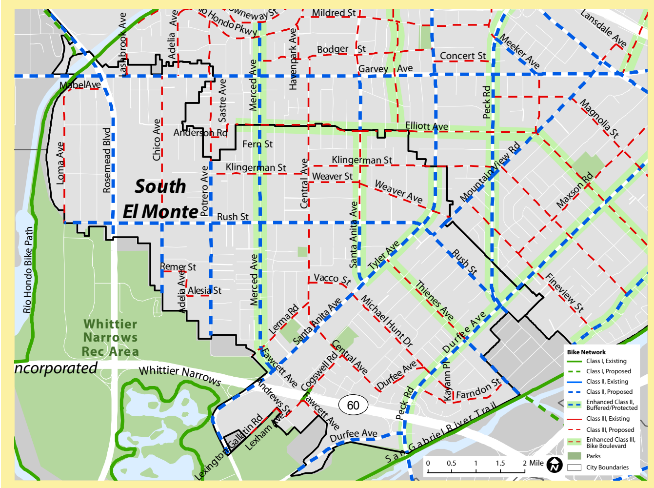
Figure 7-15 South El Monte Recommended Bikeway Network
