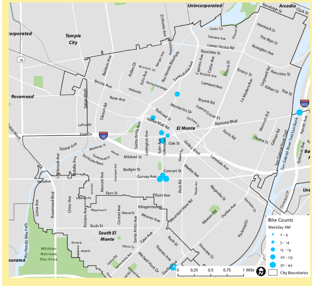
Figure 4-7 Weekday Morning Bicycle Count Results in El Monte
