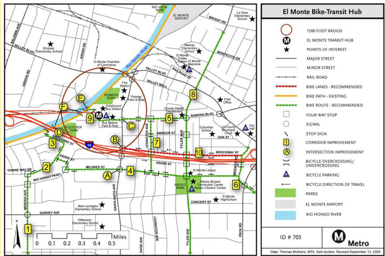
Figure 2-4 El Monte Bike-Transit Hub Recommendations
