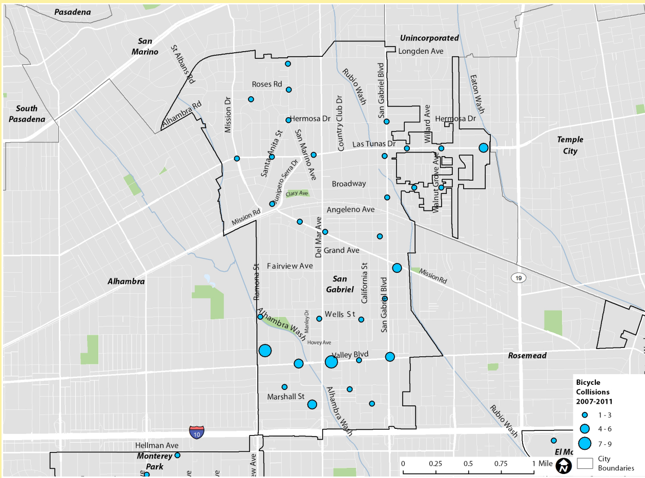
Figure 6-9 Bicycle-Related Collisions in San Gabriel, 2007-2011
